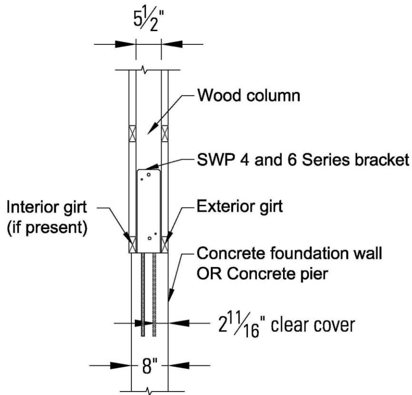
Figure 13.1: Recommended Installation For SWP 4 and 6 Series Brackets
