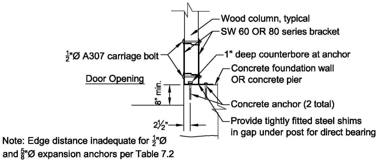
Figure 6.4: SW Door Edge Detail (Alternative)
